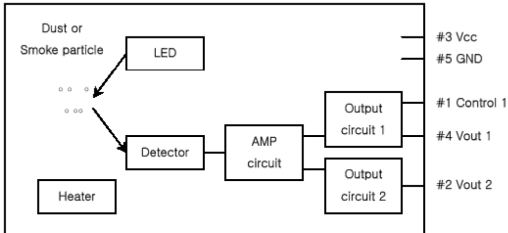
FIGURE 1.1. BLOCK DIAGRAM
